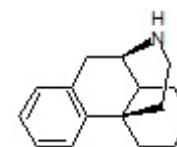
Morphinan
